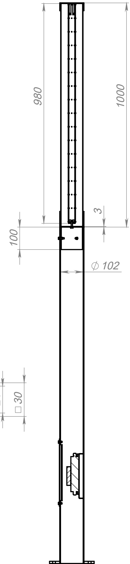
E-E (1:10)
