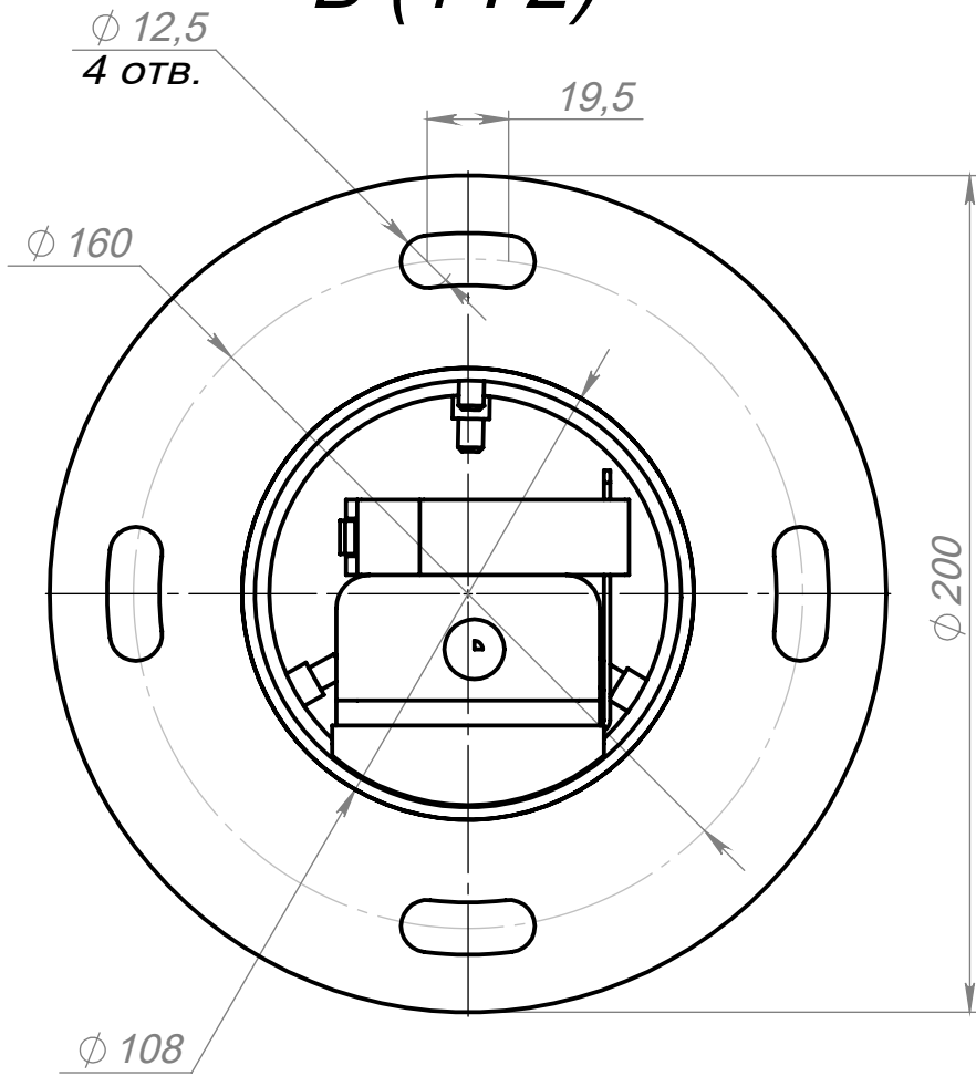
B (1:2)
